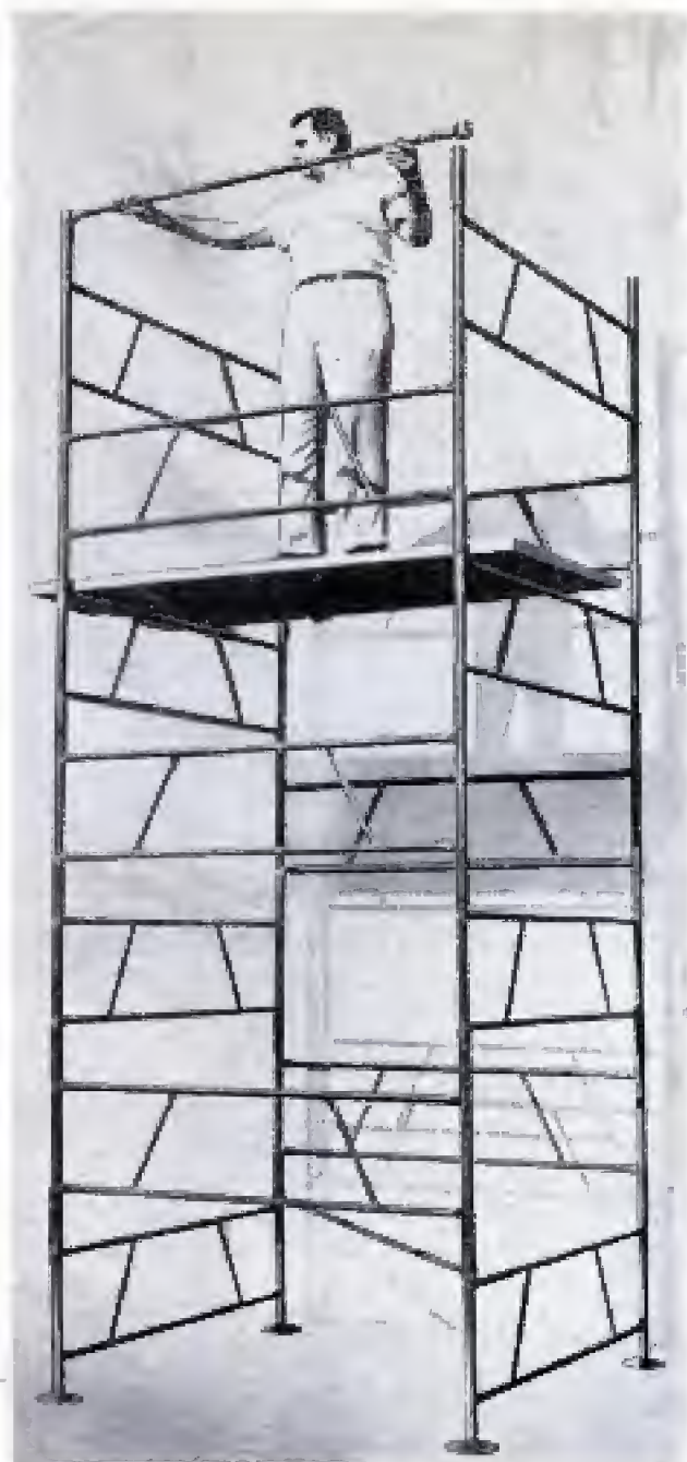
Above, 24-pound frame is basic unit of scaffolding. They slip into each other, below, to form tower, left
